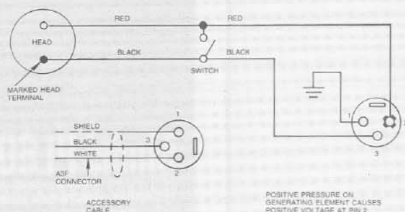
FIGURE 2 — Wiring Diagram
