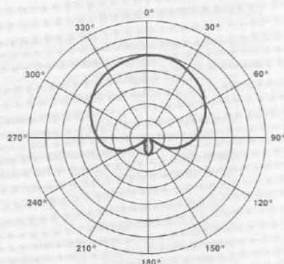
FIGURE 4 — Polar Response
