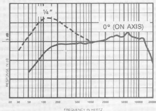
FIGURE 3 — Frequency Response
